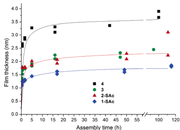
Figure 4. Growth kinetics of a series of fullerene derivatives assembled on Au in ODCB/EtOH (4:1) solvent mixtures. Film thickness was determined by ellipsometry. Compounds 1-SAc and 2-SAc were deprotected in situ using the acid deprotection method, while 3 and 4 were assembled without acid deprotection. All experiments were done under ambient conditions in a capped vessel, and the results from two separate experiments are shown for each compound.
