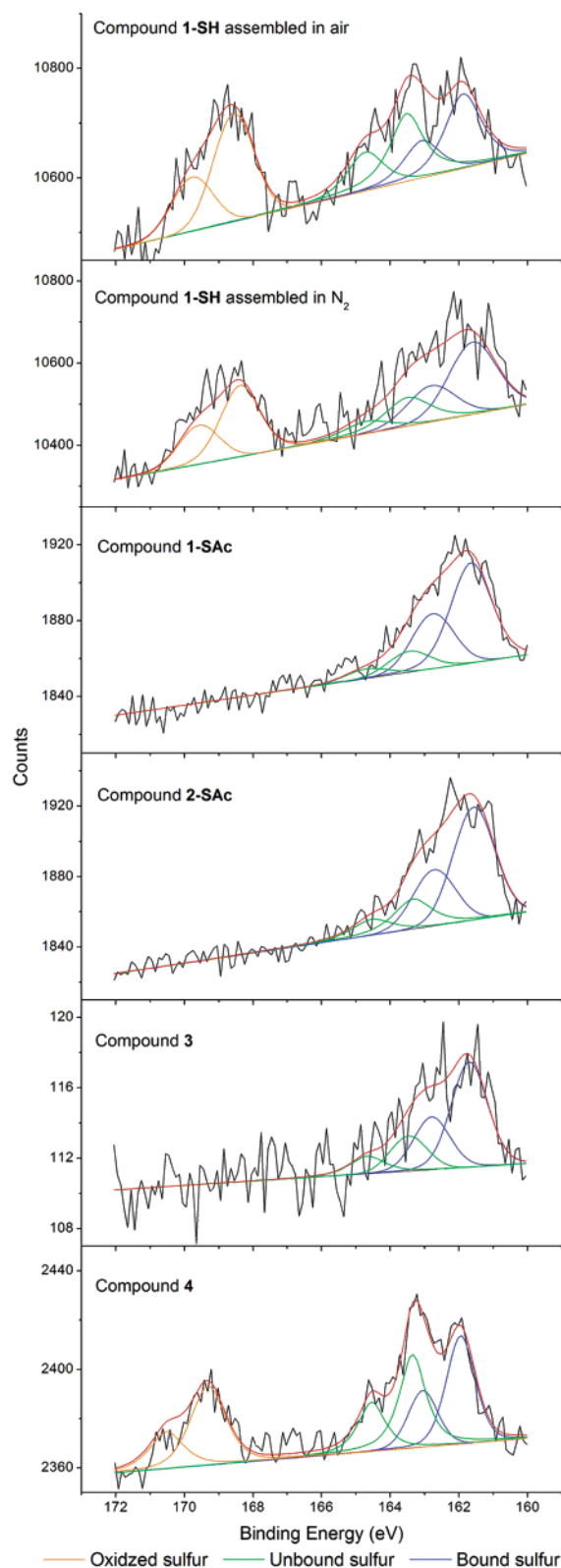
Figure 8. XPS S_{2p} spectra for 1-SH assembled using ODCB in ambient (capped vessel) or in glovebox, 1-SAc and 2-SAc assembled in ODCB/EtOH (4:1) mixture using the in situ acid deprotection method in ambient conditions, and 3 and 4 assembled in ODCB/EtOH (4:1) mixture in ambient conditions. The broad peaks from 161 to 165 eV were fit using two S_{2p} doublets with 2:1 area ratios and splittings of 1.2 eV and one S_{2p} doublet with 2:1 area ratios and splittings of 1.2 eV for the peak at \sim 169 eV. Each doublet is assigned to surface-bound, surface-unbound, and oxidized sulfur atoms.
