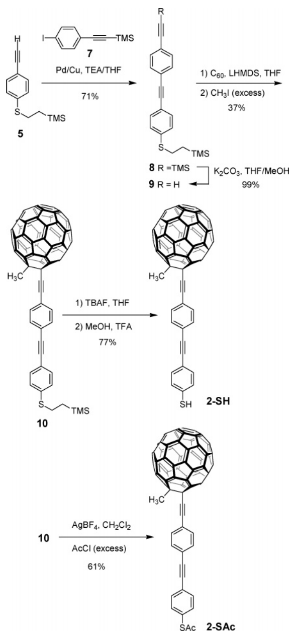
Scheme 2. Synthesis of the Fullerene–OPE Hybrids 2-SH and 2-SAc a
