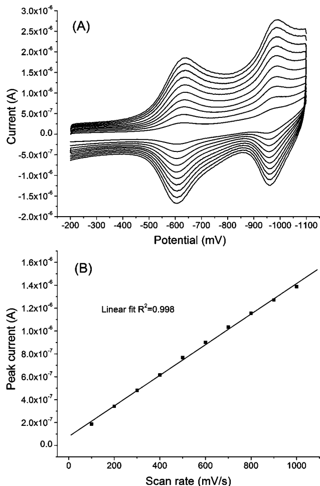
Figure 7. (A) Cyclic voltammograms of SAM of 3 on a Au bead working electrode in 0.1 M TBAPF 6 in ODCB/MeCN (4:1) at room temperature. The counter electrode was a Pt wire, and the reference electrode was Ag/AgCl. The scan rate was raised from 0.1 to 1.0 V/s with 0.1 V/s increments. (B) Peak currents at the first redox waves of part A as a function of scan rate.
